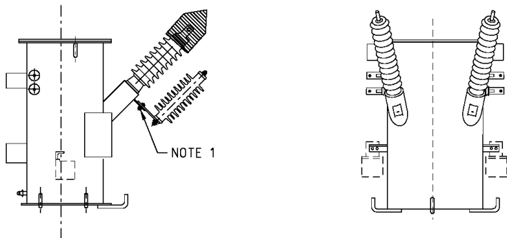
SINGLE PHASE - TWO BUSHING
