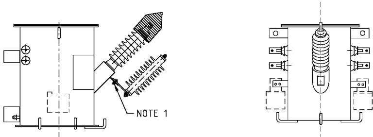
SINGLE PHASE - ONE BUSHING
