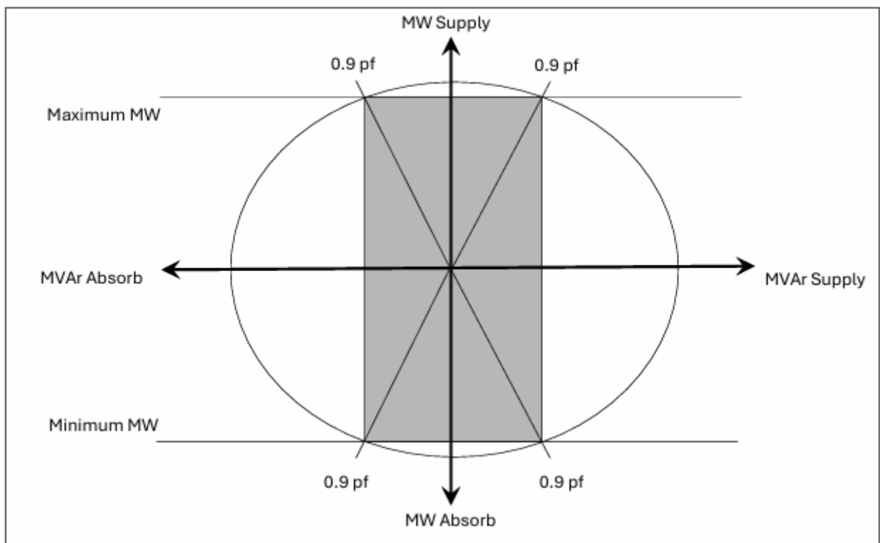
Figure 3.2 – Inverter connected generating units and induction generating units. Minimum reactive power capability requirements shown shaded
