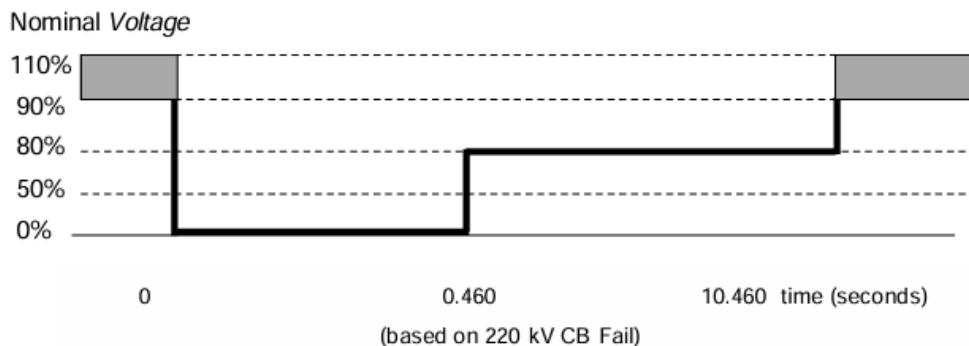
Figure 3.3 – Off nominal voltage operation capability requirement for generating units
