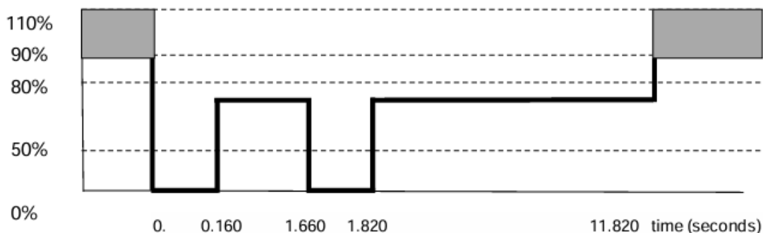
Figure 3.4 – Off nominal voltage operation capability requirement for generating units during auto-reclose operation
