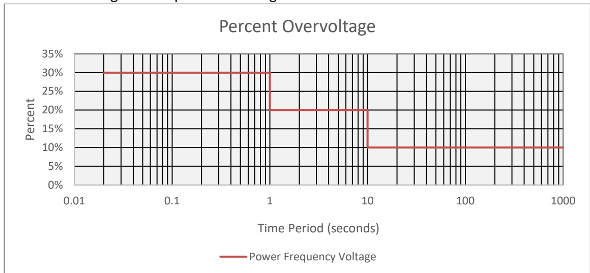
Figure 2.1 - Percentage Overvoltage Envelope
